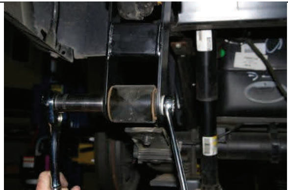
Install new shackles with OE hardware.
