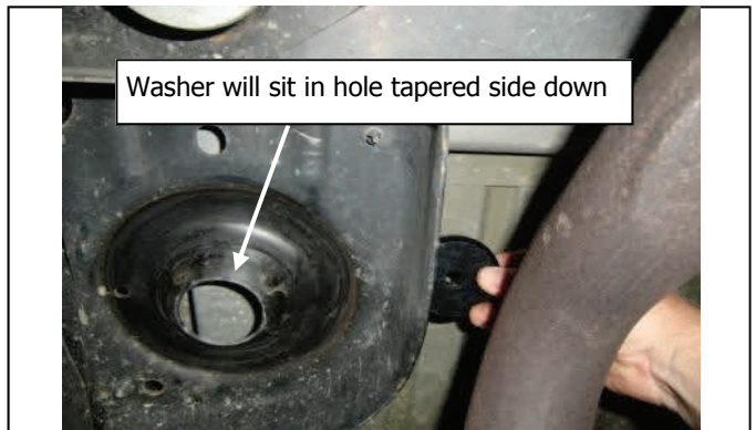
Place threaded washer above upper spring mount as shown
