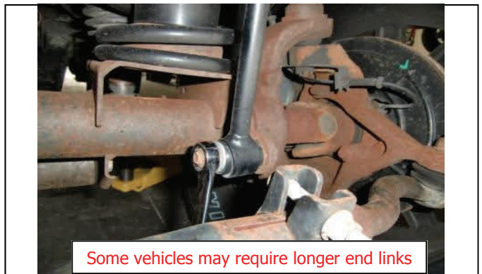
Reattach front sway bar end links .
