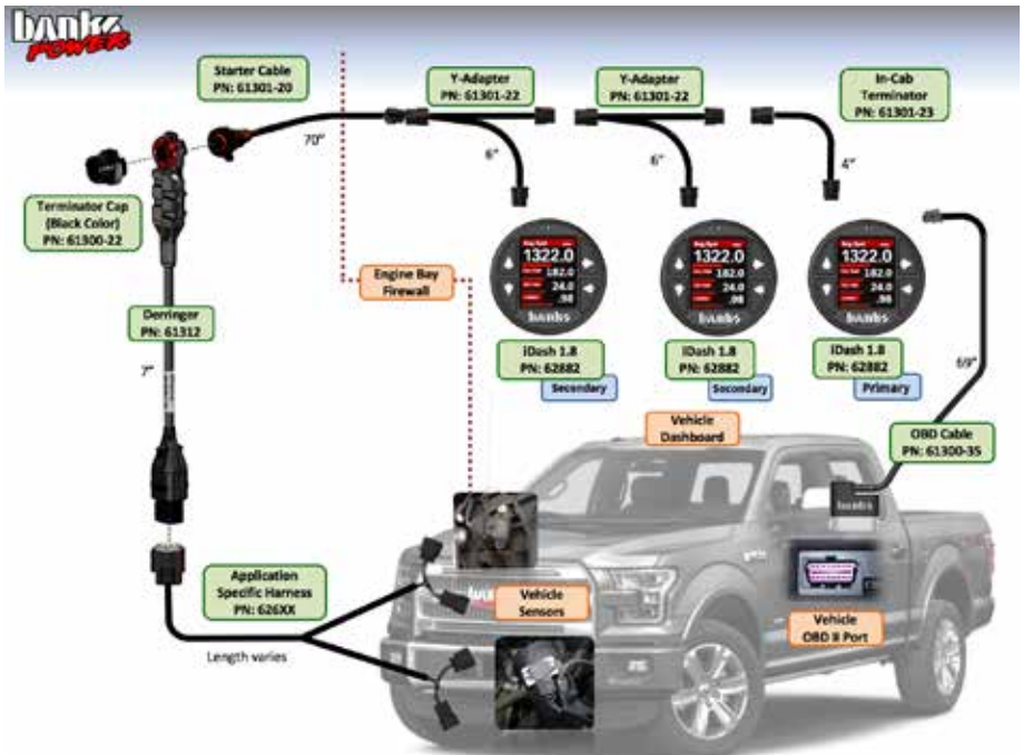
Figure 6 – Daisy Chain
