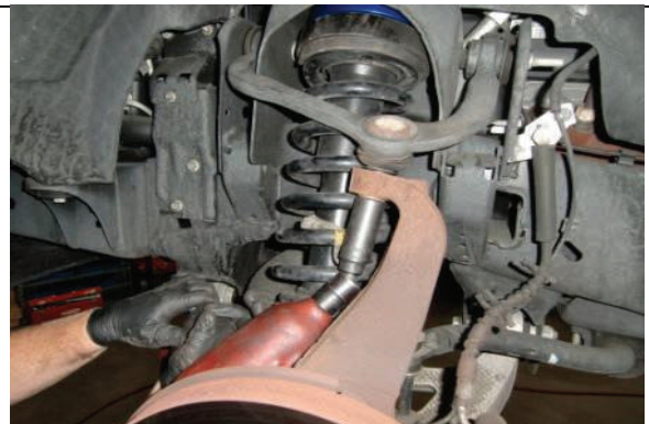
Tighten upper ball joint nut to spec
