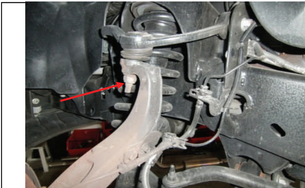
Loosen but do not remove upper ball joint nut
