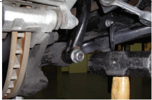
Strike with hammer to loosen bolt from lower control arm
